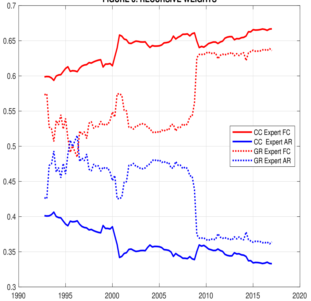
FIGURE 8: RECURSIVE WEIGHTS
