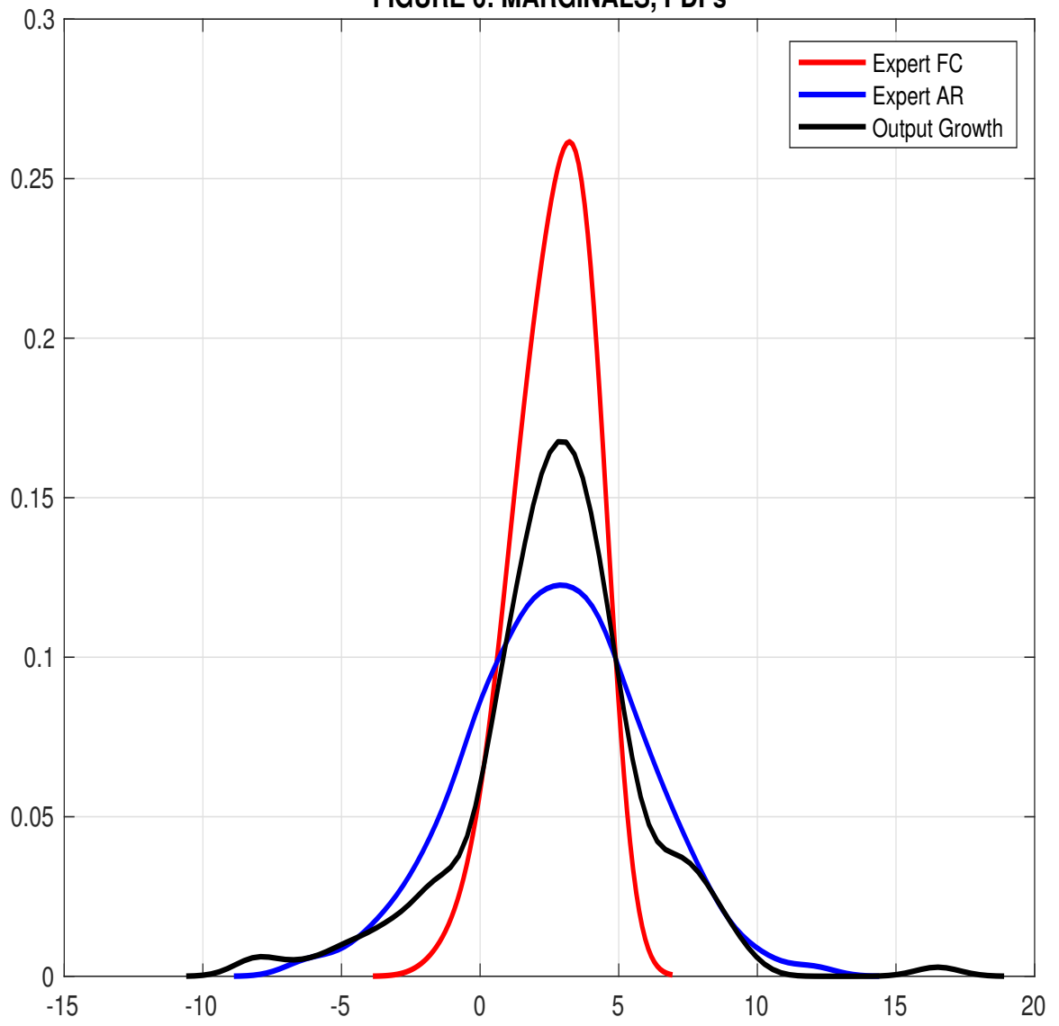
FIGURE 6: MARGINALS, PDFs
