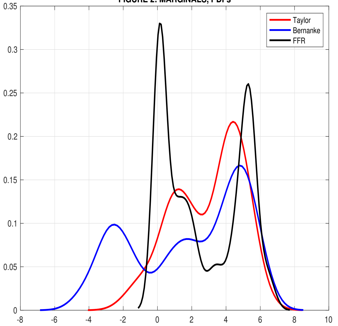
FIGURE 2: MARGINALS, PDFs
